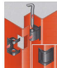
Cut-out hinge example
